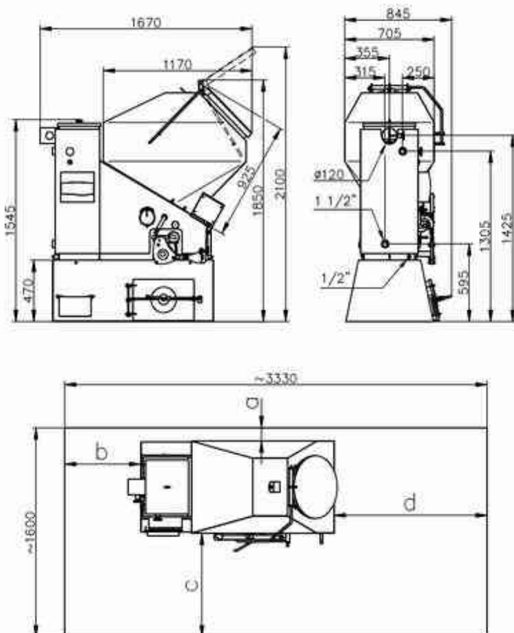
CARBOROBOT Classic 40
